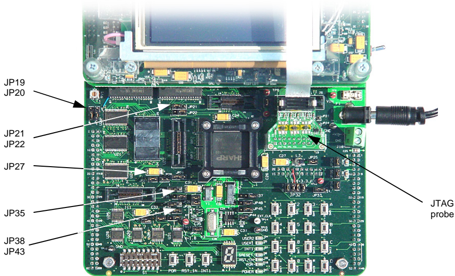
FIGURE 3 Sharp KEV75401 Evaluation Board.
